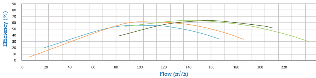
Hydraulic Performance
