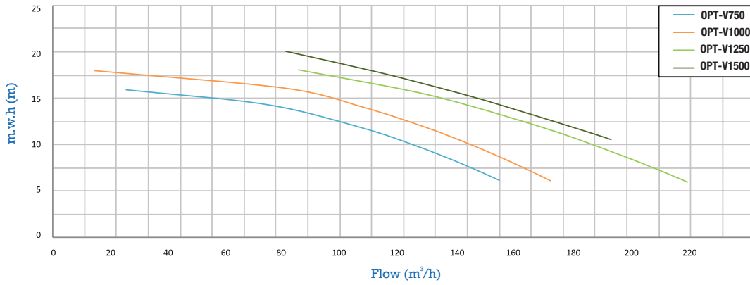
Hydraulic Performance
