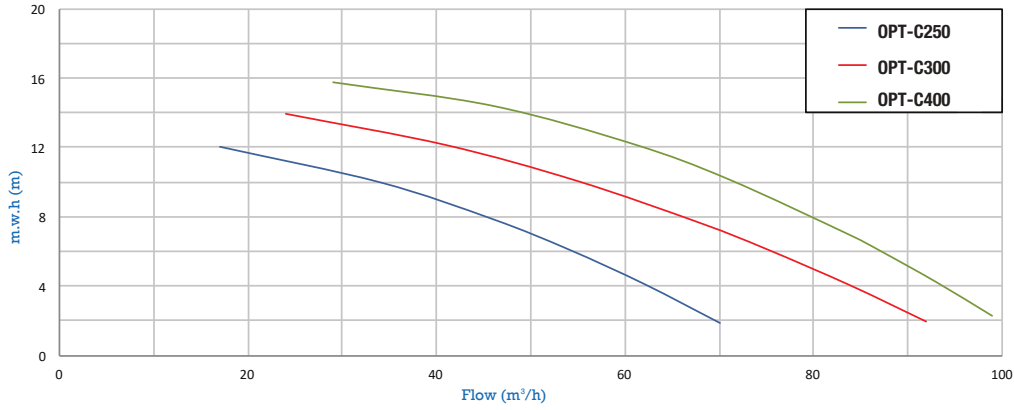
Characteristics curve
