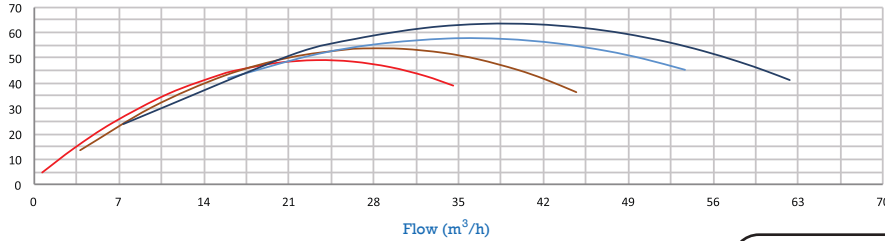
Hydraulic Performance
