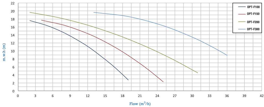
Characteristics curve
