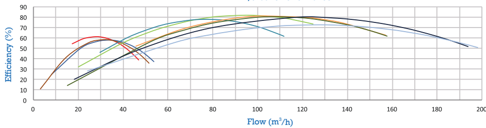
Hydraulic Performance
