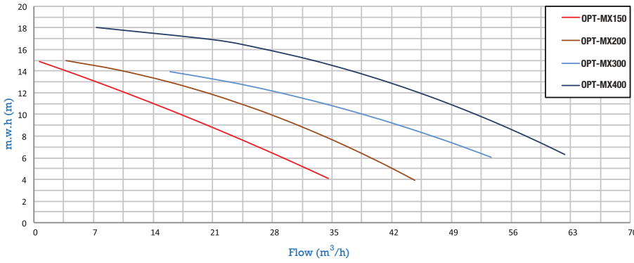
Characteristics curve
