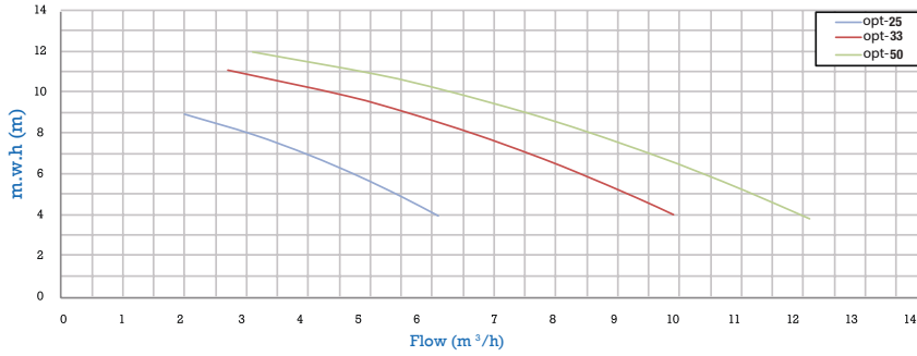
Characteristics curve
