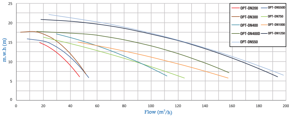
Hydraulic Performance
