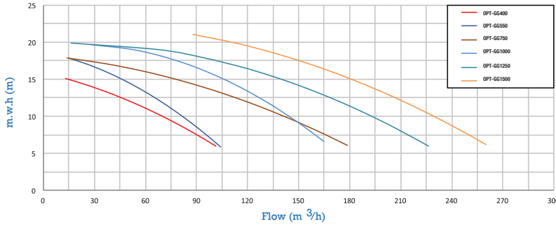
Hydraulic Performance
