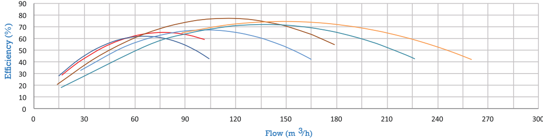
Hydraulic Performance
