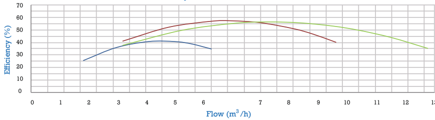
Hydraulic Performance
